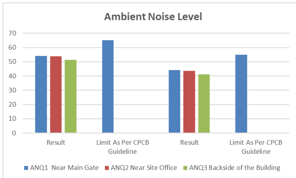
Figure 3.1 Location-wise Variation of Ambient Noise Levels
